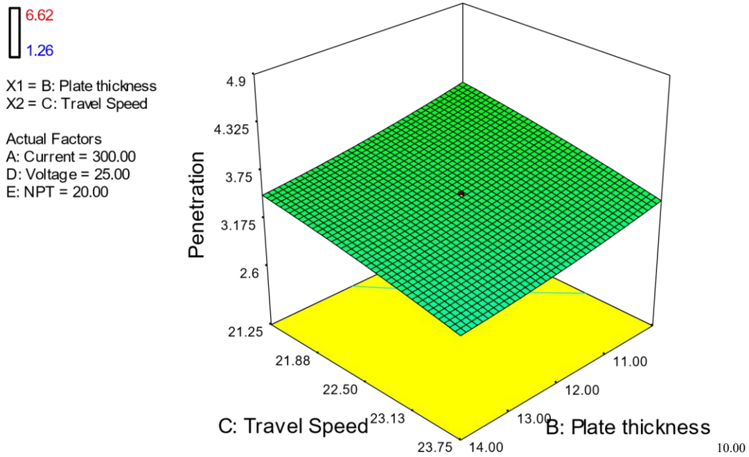
Fig. 2 3D plot for the effect of travel speed and plate thickness on Penetration
