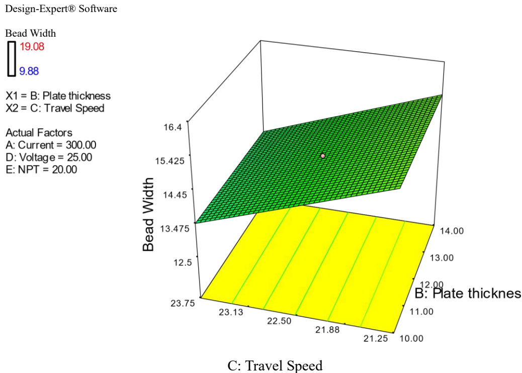
Fig. 6 3D plot for the effect of travel speed and plate thickness on bead width
