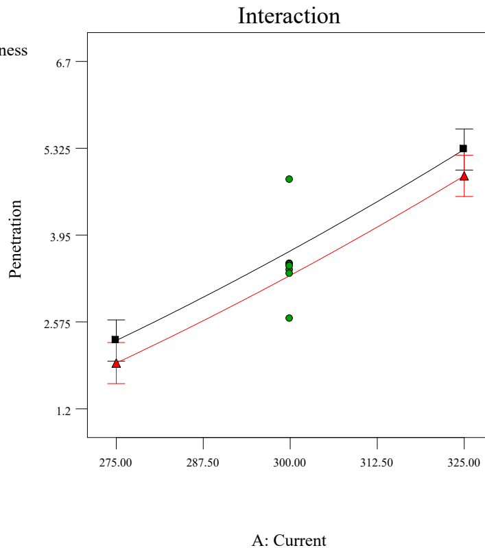
Fig. 3 Interaction effect of current and plate thickness on penetration
