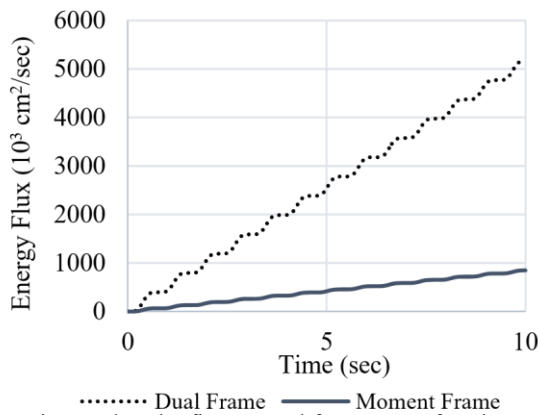
Fig. 12 Sweep wave loading
