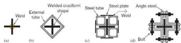
Fig. 2 Common cross-sections for steel BRB
