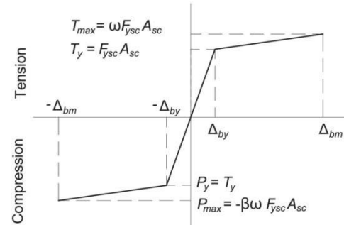
Fig. 9 BRB force-deformation bi-linear
