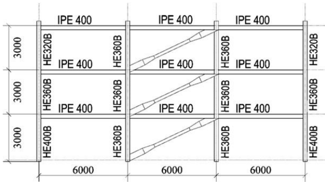
Fig. 8 Dual moment steel frame with BRB
