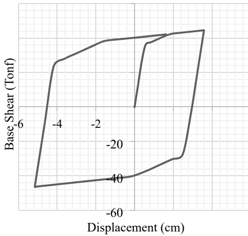
Fig. 18 Single BRB hysteresis curve
