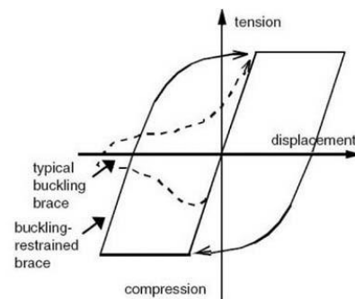
Fig. 3 Force-displacement behavior between BRB and traditional braces
