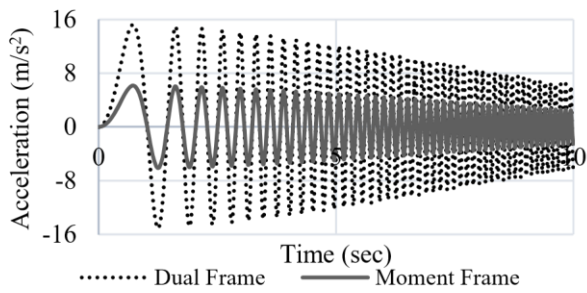
Fig. 12 Sweep wave loading
