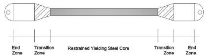
Fig. 1 BRB components
