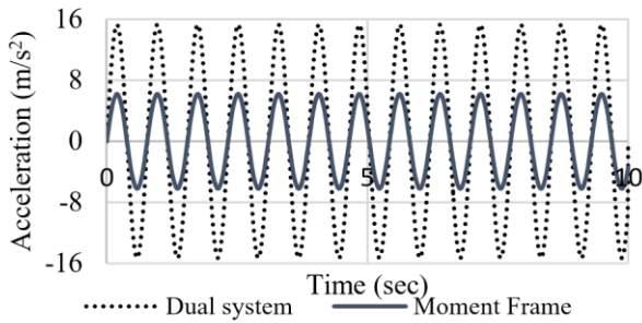
Fig. 11 Harmonic loading
