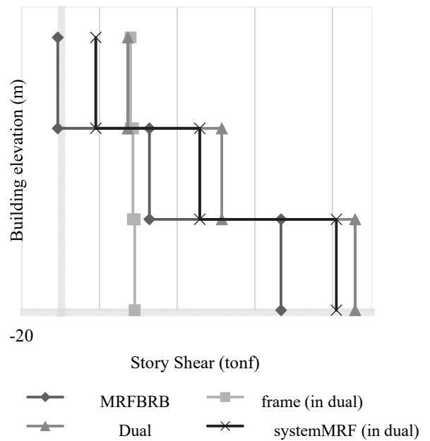
Fig. 17 Story shear distribution over height
