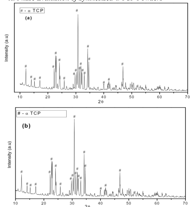
Fig. 1 X-ray diffraction pattern of as synthesized \alpha TCP powders (a) undoped (b) Si doped
