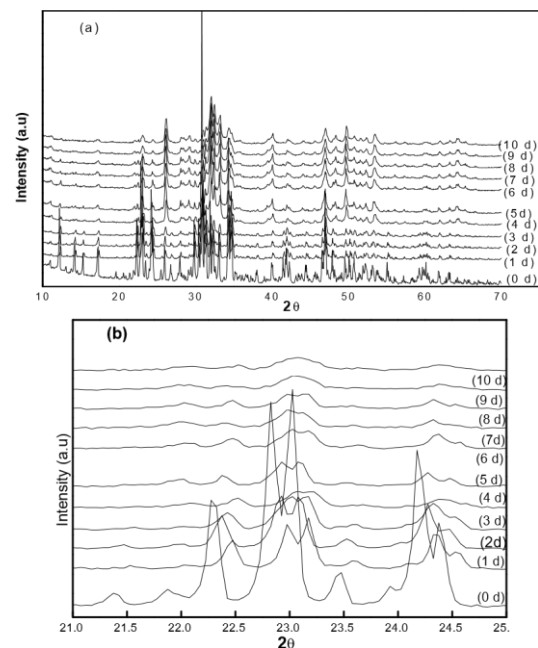
Fig. 3 XRD pattern of Si doped CPC in SBF with 2\theta varying from (a) 10-70^\circ (b) 20-25^\circ
