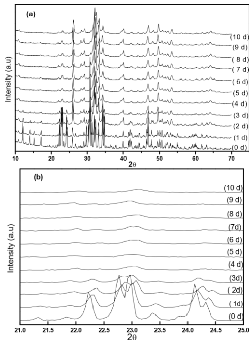
Fig. 2 XRD pattern of undoped CPC in SBF with 2\theta varying from (a) 10-70^\circ (b) 20-25^\circ
