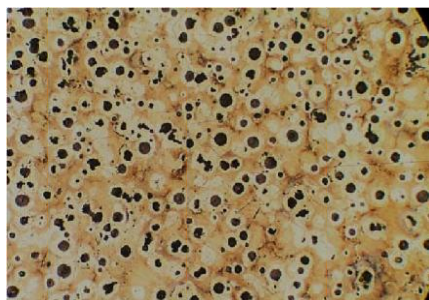
(b) Nodular iron with 0.5 % Cu
