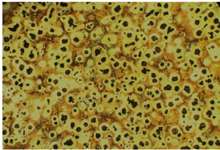
(a) Nodular iron without Cu
