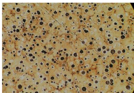
(c) Nodular iron with 1.2 % Cu
