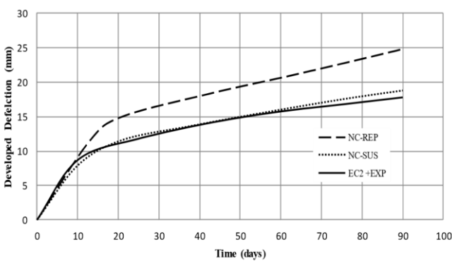
Fig. 4 (a) Mid-Span Deflection with Time (NC-SUS, EC2 and Midas FEA), (b) Mid-Span Deflection with Time (NC-REP, NC-SUS and
