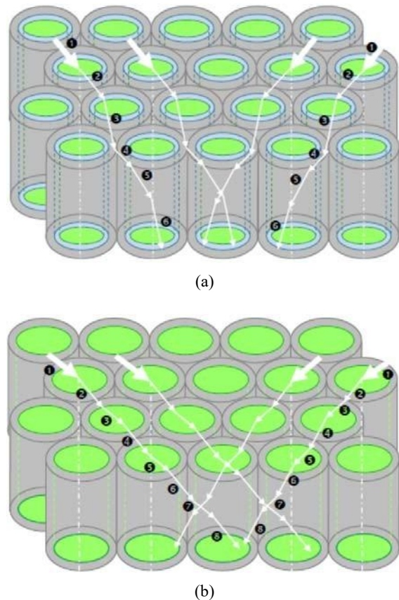
Fig. 3 Light refraction path in the (a) CsI/AAO and (b) CsI/TiO 2 /AAO composites. A higher refractive index material of TiO 2 film reduces the refraction path from the CsI top to the bottom
