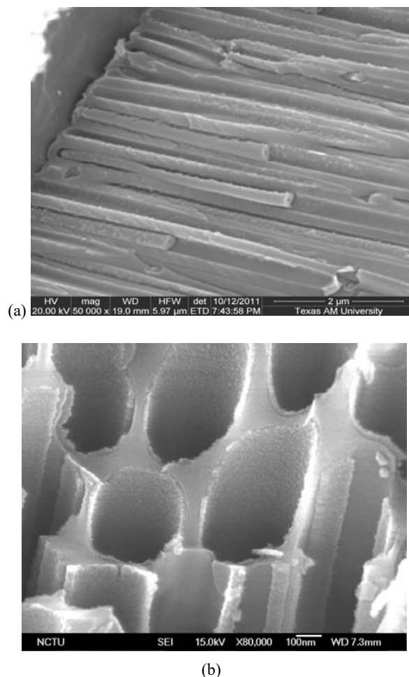
Fig. 5 SEM images of \text{TiO}_2 forming in/on the AAO pore wall; (a) \text{TiO}_2 tube forming inside AAO tube under 0.2 wt.% \text{TiF}_4 solution for 2 h conditions, (b) \text{TiO}_2 film coating on the AAO tube under 0.01 wt.%
