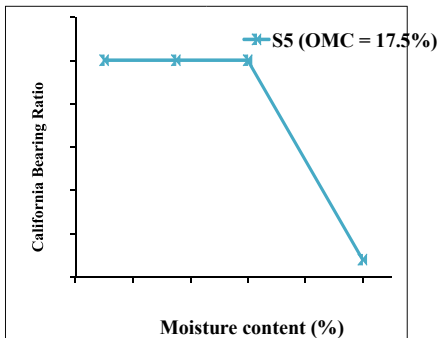
Fig. 2 (e) The CBR versus the moisture content for soil sample S5
