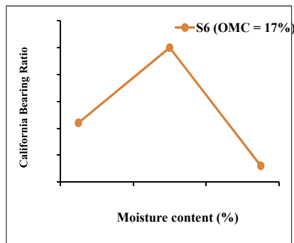
Fig. 2 (f) The CBR versus the moisture content for soil sample S6
