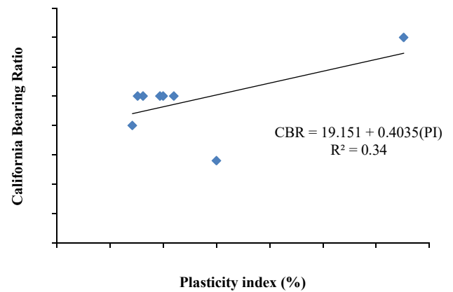
Fig. 3 Plasticity index versus CBR for the experimental soil samples at OMC
