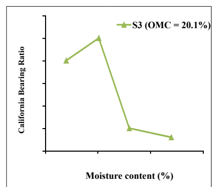
Fig. 2 (c) The CBR versus the moisture content for soil sample S3
