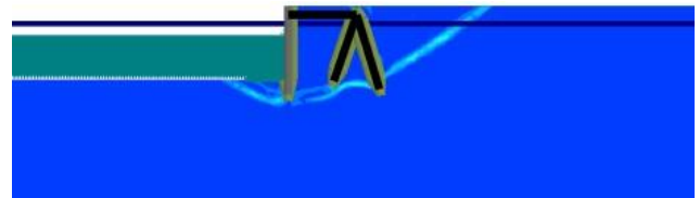
Fig. 11 Failure plane at critical acceleration as computed with PLAXIS 2D
