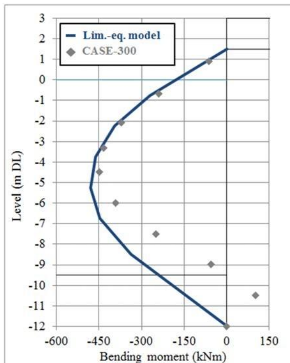
Fig. 13 Bending moment line computed with the limit-equilibrium model compared with the reference case measurements
