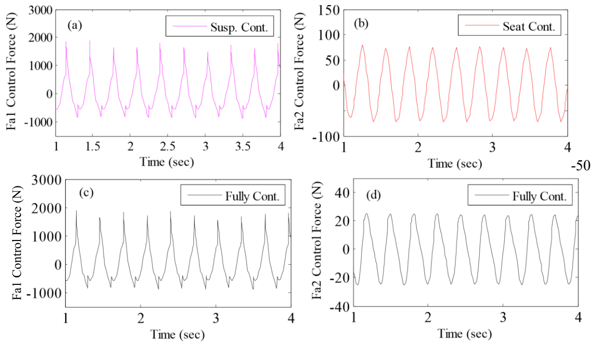
Fig. 12 Control force supplied by HFPIDCR controller in suspension system (a) Suspension controlled; (b) Passenger seat controlled; (c) Fully
