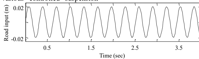
Fig. 9 Sinusoidal road profile
