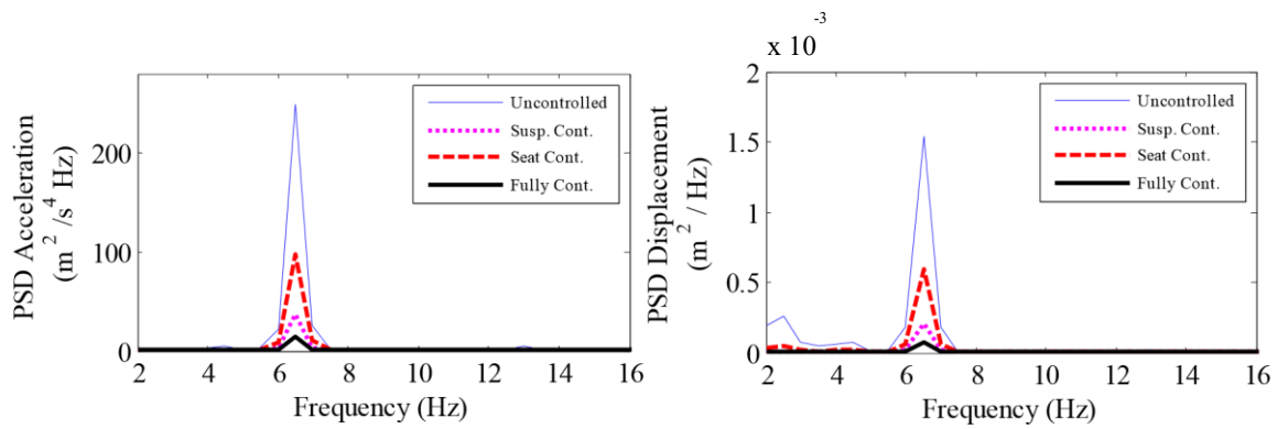
Fig. 11 PSD of passenger seat acceleration, passenger seat displacement
