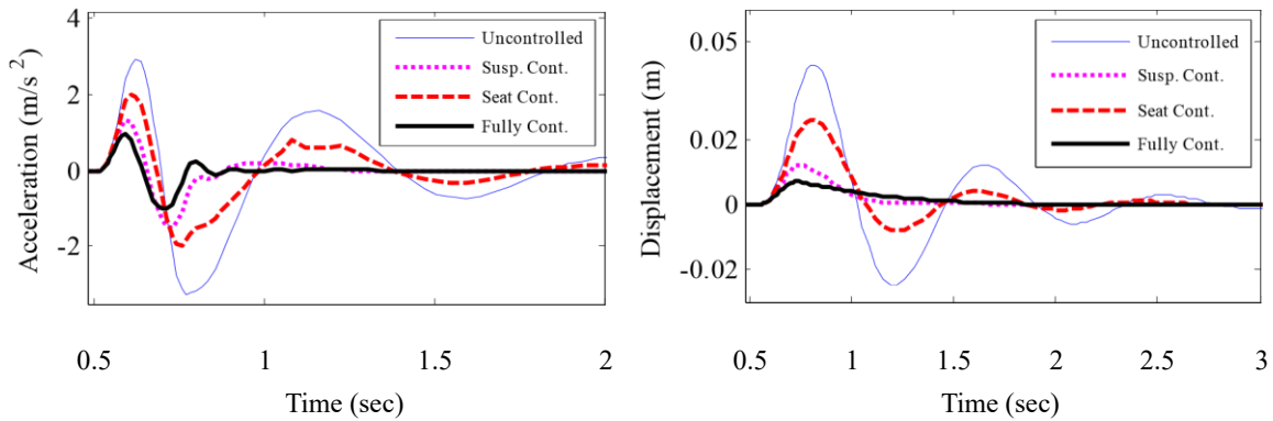
Fig. 6 Bump response of passenger seat acceleration, passenger seat displacement
