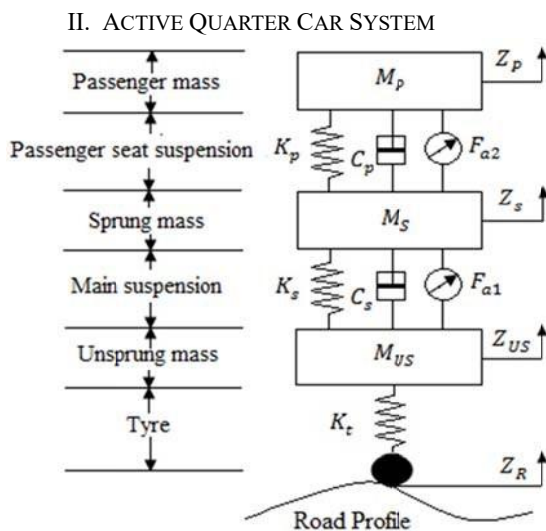
Fig. 1 Active quarter car suspension system
