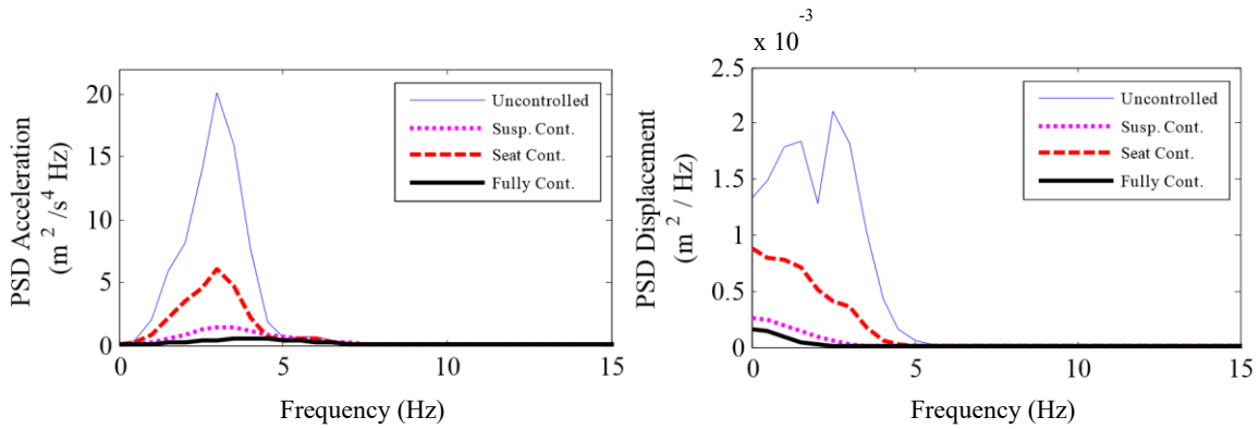
Fig. 7 PSD of passenger seat acceleration, passenger seat displacement
