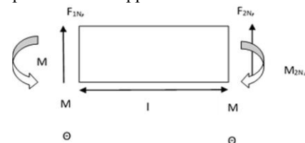
Fig. 1 Beam element with generalized forces and displacement
