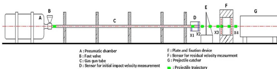
Fig. 1 Experimental device presentation
