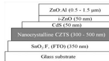
Fig. 4 Nanocrystalline development in CZTS solar cell [15]
