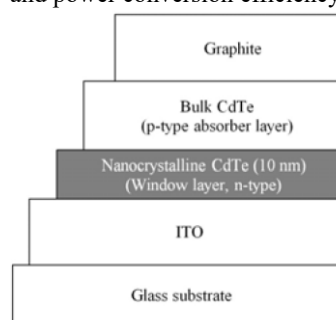
Fig. 1 Nanostructured development in CdTe Solar Cell [11]
