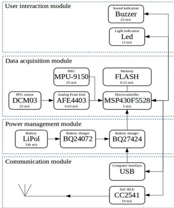
Fig. 3 Structure and basic components of the developed monitoring device
