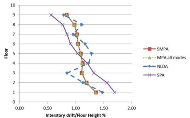
Fig. 22 Inter-story drift/Floor Height % comparison for Loma Prieta the use of NLDA. In this thesis, the SMPA is presented and used in the analysis. To validate the SMPA method, a comparison between the techniques has been done and related to the most accurate technique which is the NLDA. The methods are introduced and used to compute the values of the floor displacements, base shear, and inter-story drifts.
