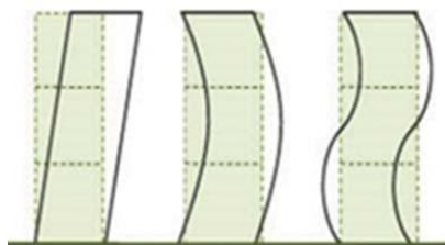
Fig. 1 First, second, and third modes of vibration
