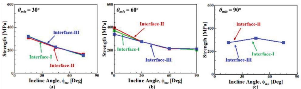
Fig. 2 Strength vs incline angle with different types of interface (a) mismatch angle =30°, (b) mismatch angle =60°, and (c) mismatch angle =90°
