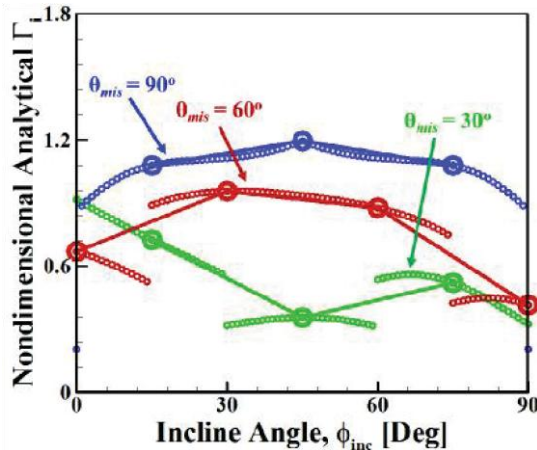
Fig. 5 Analytical approximation of the energy release rate for delamination ( \Gamma_i ) as a function of incline angle ( \phi_{inc} ) for the structures with mismatch angle =30°, 60° and 90°
