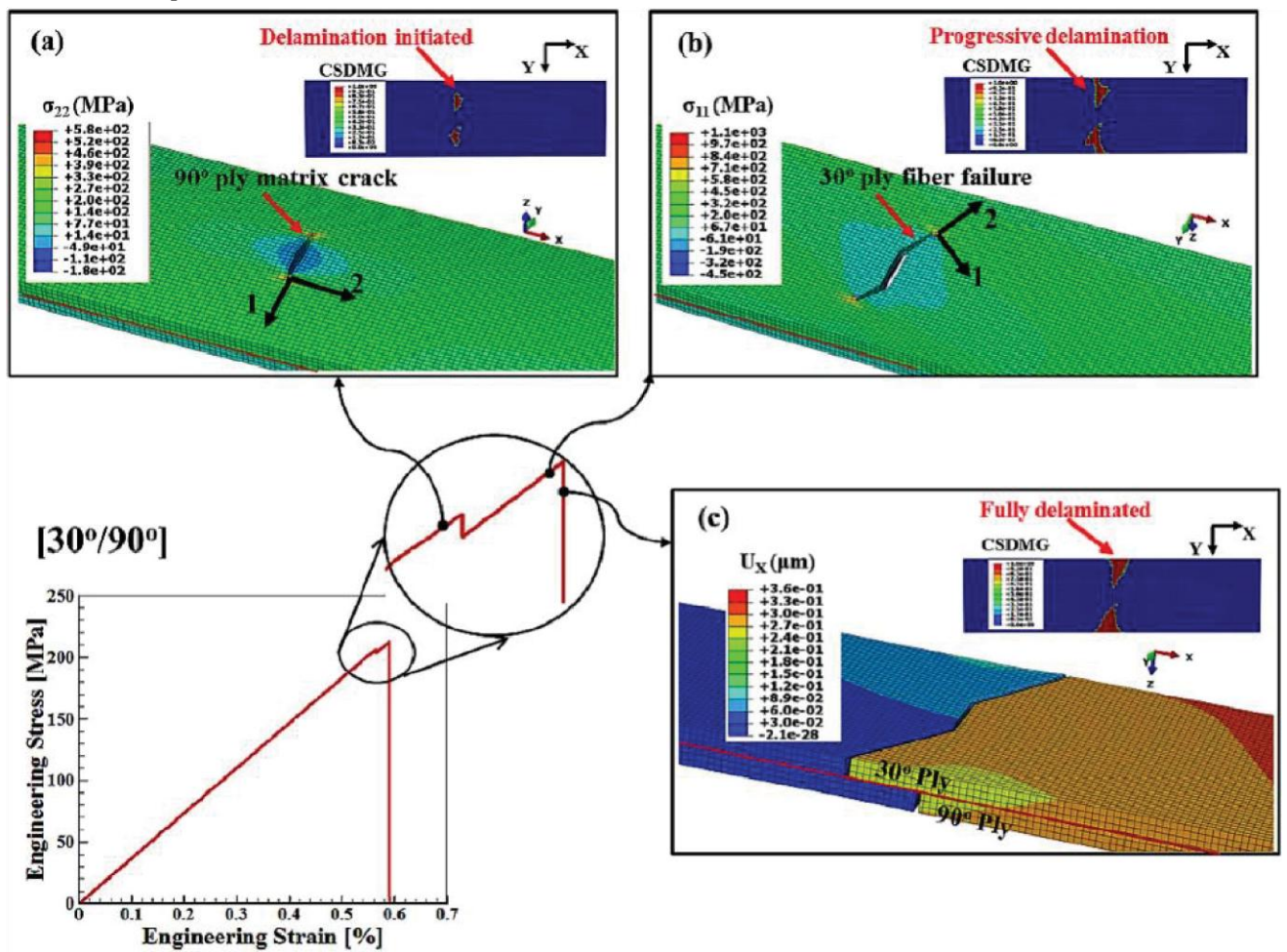
Fig.1 Engineering stress-strain curve for the [30°/90°] example with simulation snapshots for the progressive damage in the laminated structure (a) matrix crack on the 90°ply, (b) fiber failure on the 30°ply, (c) the final status of the damage process
