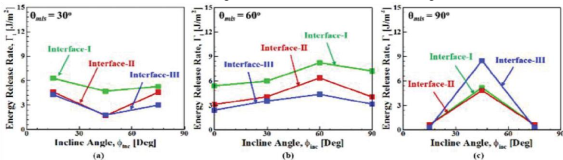
Fig. 4 Energy release rate for delamination ( \Gamma_i ) as a function of incline angle ( \phi_{inc} ) with different types of interfaces for (a) mismatch angle = 30^\circ , (b) mismatch angle = 60^\circ , and (c) mismatch angle = 90^\circ
