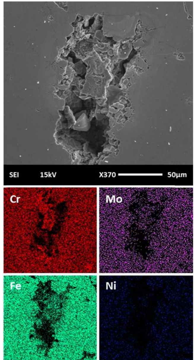
Fig. 7 SEM image and X-ray mapping results of formed pit on the coating after corrosion test
