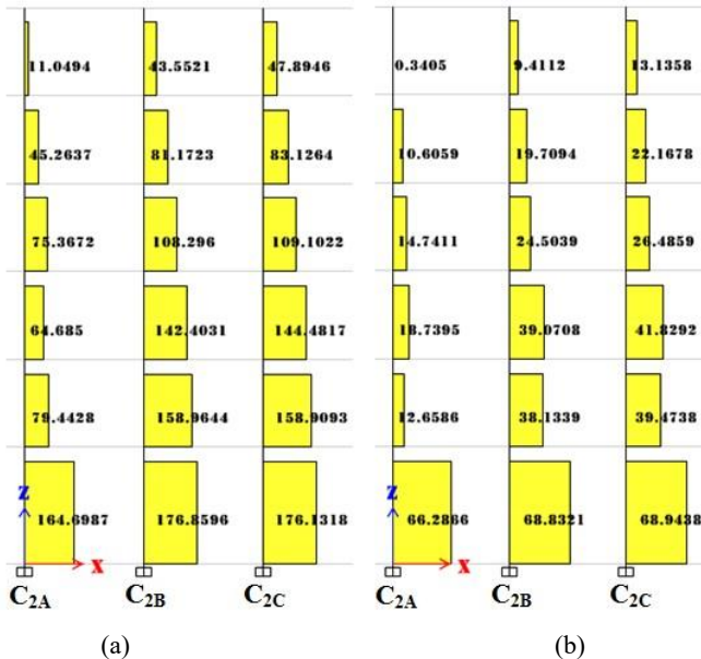
Fig. 8 Column shearing force distribution for two models (a) bare frame (b) masonry infill frame
