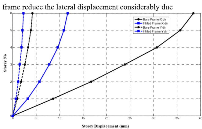
Fig. 5 Storey displacements in X and Y direction throughout the height of building for two building models under RS loading in X-dir
