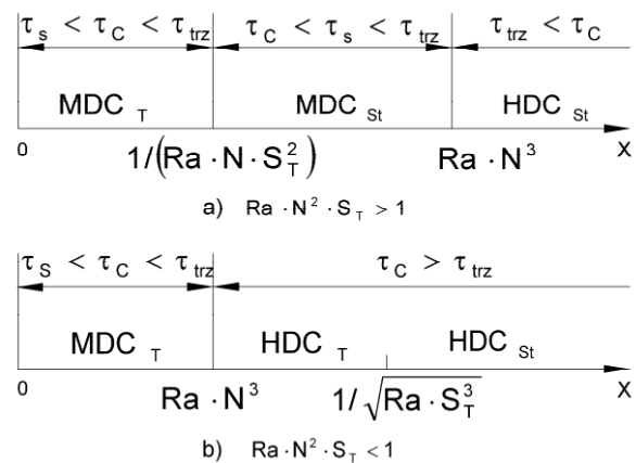
Fig. 2 The heat and mass driven natural convection regimes sequence a) Ra \square N^2 \square S_T \square I ; b) Ra \square N^2 \square S_T \square I
