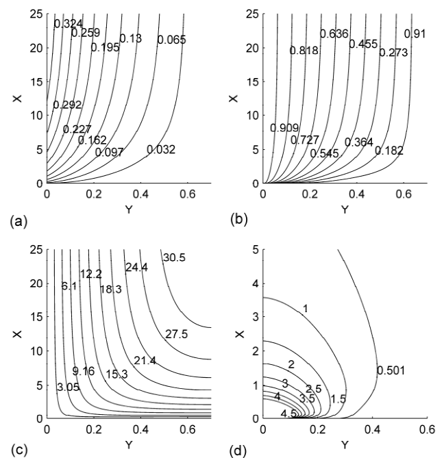
Fig. 3 (a) Dimensionless temperature \theta , (b) concentration \phi , (c) stream function \psi and (d) \psi/\sqrt{X} fields Ra = 300 ,
