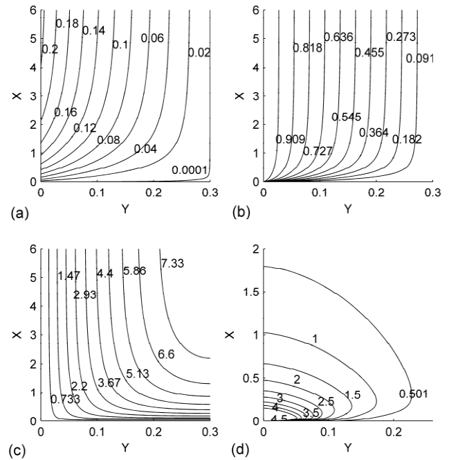
Fig. 7 (a) Ra , (b) N , (c) Le , and (d) Sr fields. Ra = 600 , N = 0.2 , Le = 1 and Sr = 0.05
