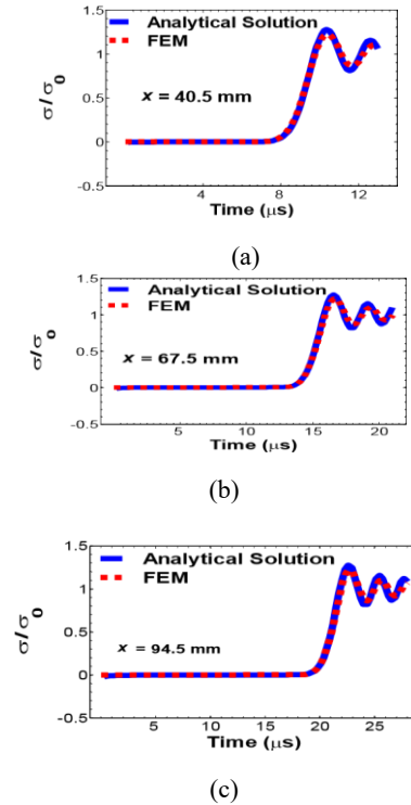
Fig. 3 Comparison of stress wave profiles obtained from FEM with those calculated from theoretical work [39] for (a) x = 40.5 mm, (b) x = 67.5 mm, (c) x = 94.5 mm ( d = 1.5 mm, b = 1.2 mm, E_h = 108
