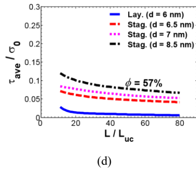
Fig. 8 Comparison of average (a) normal, (b) shear stress in vertically layered and staggered structure and comparison of average (c) normal, (d) shear stress in horizontally layered and staggered structure for mineral volume fraction of 57% ( E_m=130 GPa, E_c=1 GPa, v_m=v_c=0.28 , \rho_m=2 g/cm 3 , \rho_c=1 g/cm 3 )
