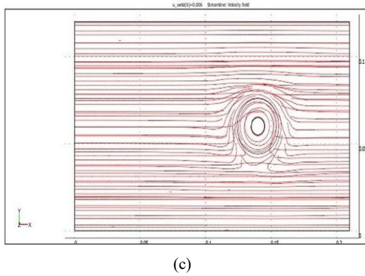
Fig. 7 Flow pattern for various tool traverse speed, (a) 0.002 ms -1 , (b) 0.004 ms -1 and (c) 0.006 ms -1 for rotational speed of 400 rpm, full sticking condition and coefficient of friction 0.4
