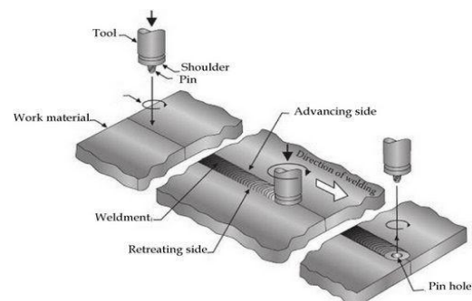
Fig. 1 Schematic diagram of friction stir welding process [2]
