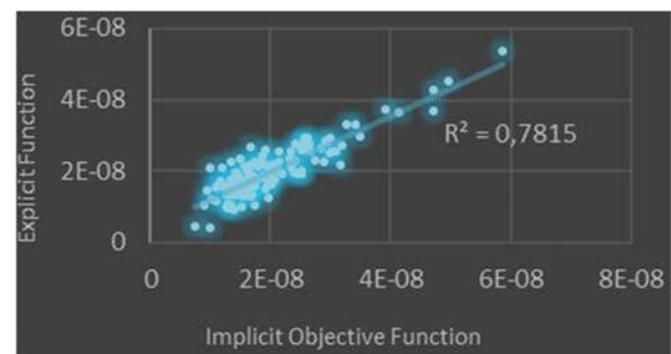
Fig. 22 Correlation between weight implicit and explicit objective functions for third case study with SMF
