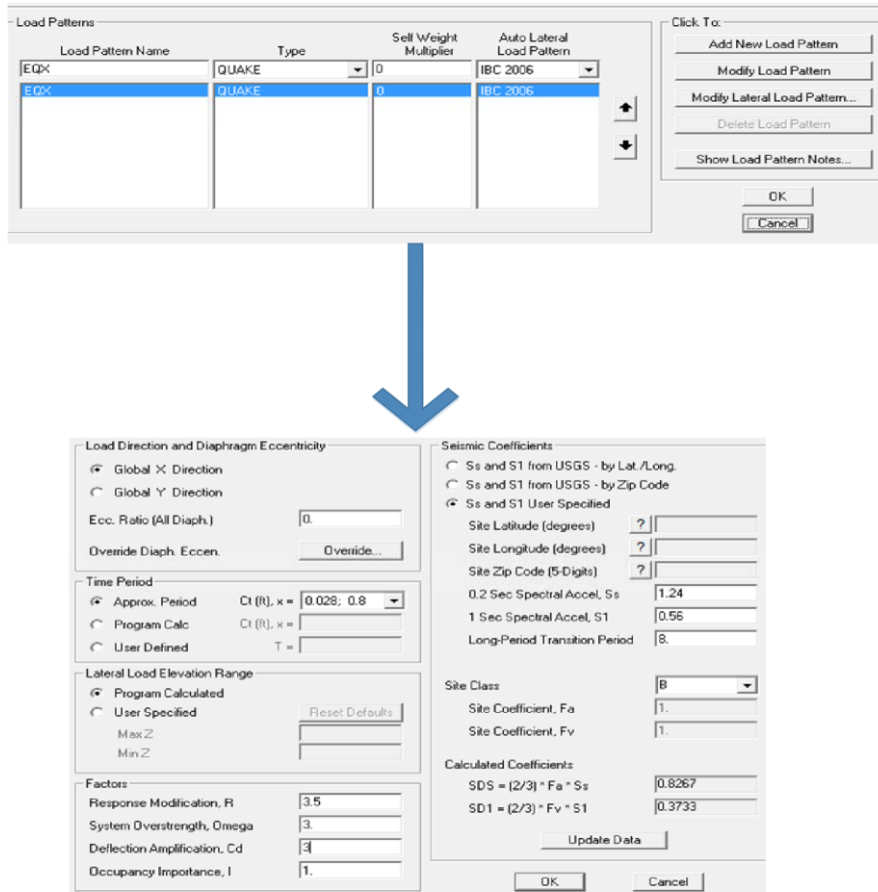
Fig. 3 Seismic load simulation in SAP software
