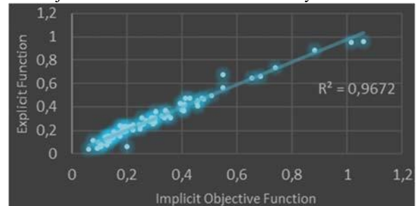
Fig. 17 Correlation between relative cost implicit and explicit objective functions for second case study with IMF
