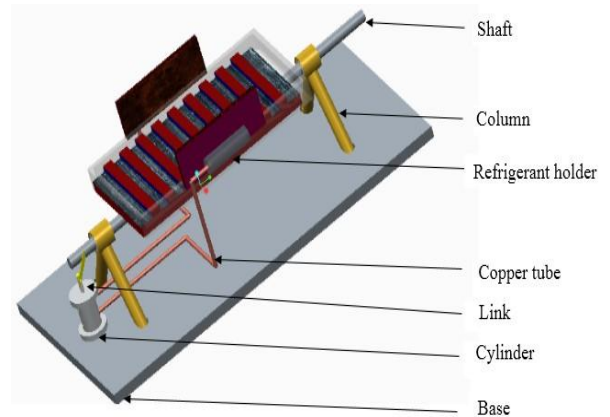
Fig. 5 Model of Solar Tracking System with Refrigerant
