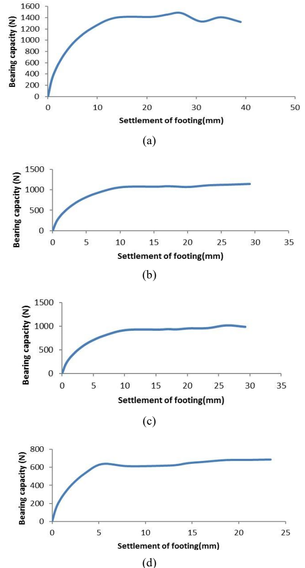
Fig. 4 Load-settlement curves for various load eccentricity: (a) e=0 (b) e=0.75 \text{ cm} (c) e=1.5 \text{ cm} (d) e=2.25
