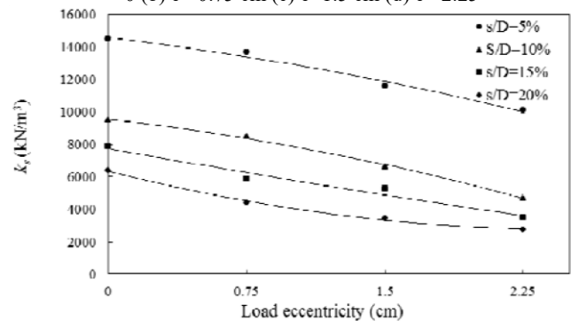
Fig. 5 Modulus of subgrade reaction versus the load eccentricity
