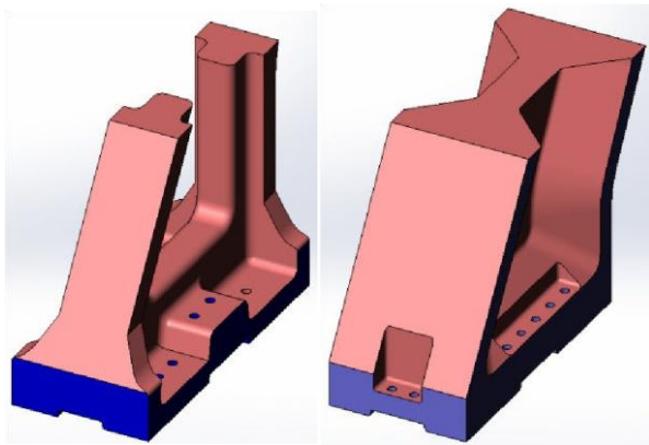
(a) Initial designs (b) Final designs Fig. 5 Columns geometry and dimension modification
