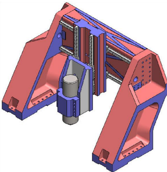
(a) Initial designs (b) Final designs Fig. 5 Columns geometry and dimension modification
