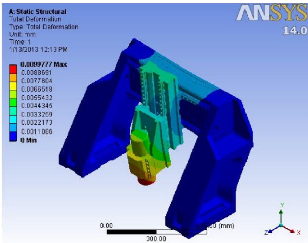
Fig. 11 The static analysis result
